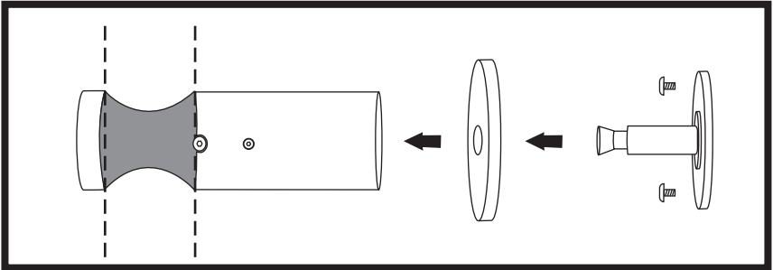
Bracket assemble - Top view
